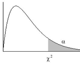
For d.f. \geq 3
