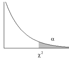
For d.f. = 1 or 2
